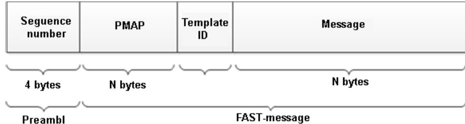
Pic. 3. Message structure
