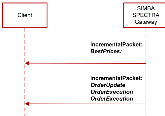
Fig. 7. Diagram. Updating - empty order-book
